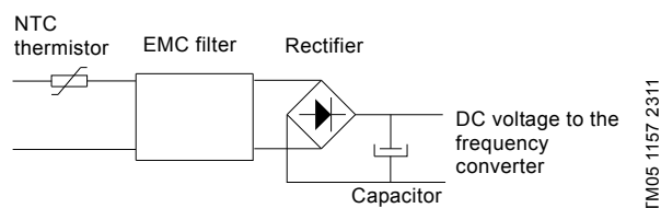
Fig. 23 Rectification of VAC voltage to DC voltage
