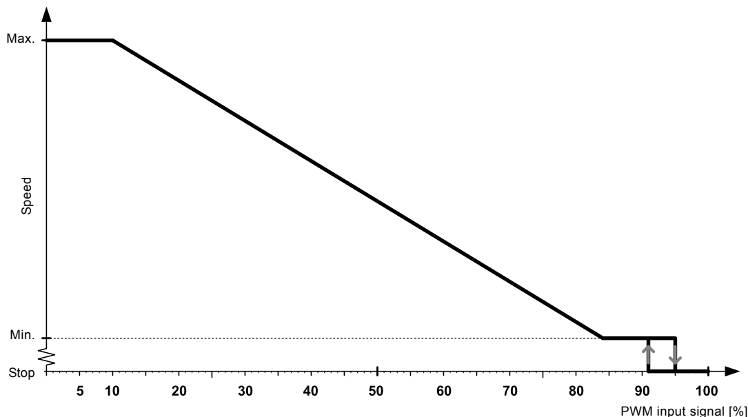
Fig. 6 PWM input profile HEATING
