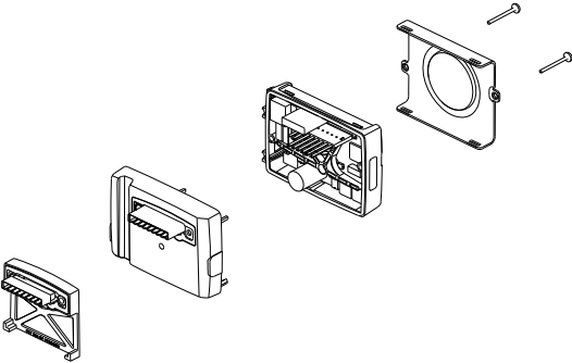
Fig. 22 Control box
