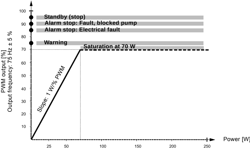
Fig. 7 PWM feedback signal, UPM2 and UPM2K
