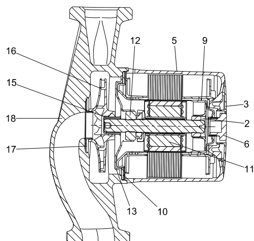
Fig. 11 UPM2, UPM GEO and UPM2K
