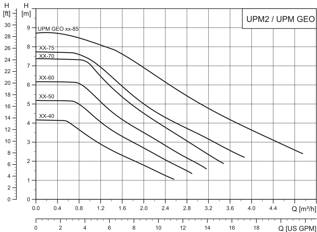
Fig. 2 UPM2 and UPM GEO
