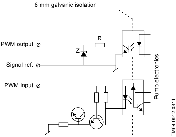
Fig. 5 Schematic drawing, interface
