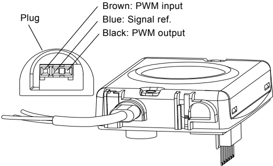
Fig. 25 Signal cable
