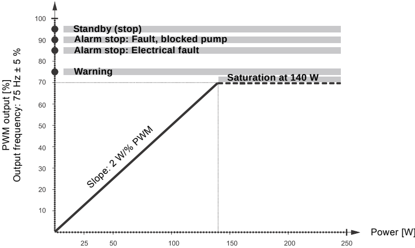
Fig. 8 PWM feedback signal, UPM GEO
