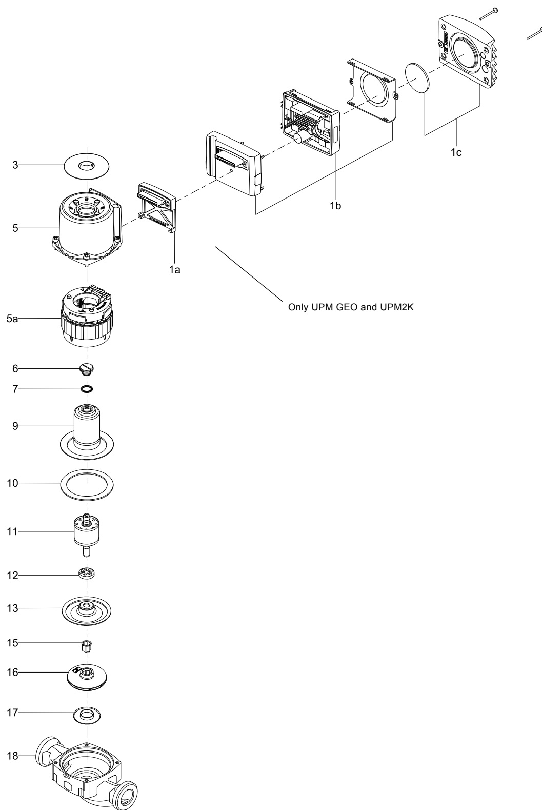
Fig. 10 UPM2, UPM GEO and UPM2K
