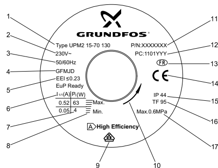
Fig. 1 Nameplate
