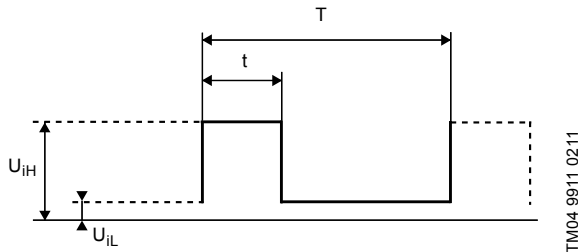
Fig. 4 PWM signal
