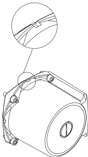
Fig. 13 Drain hole in stator housing
